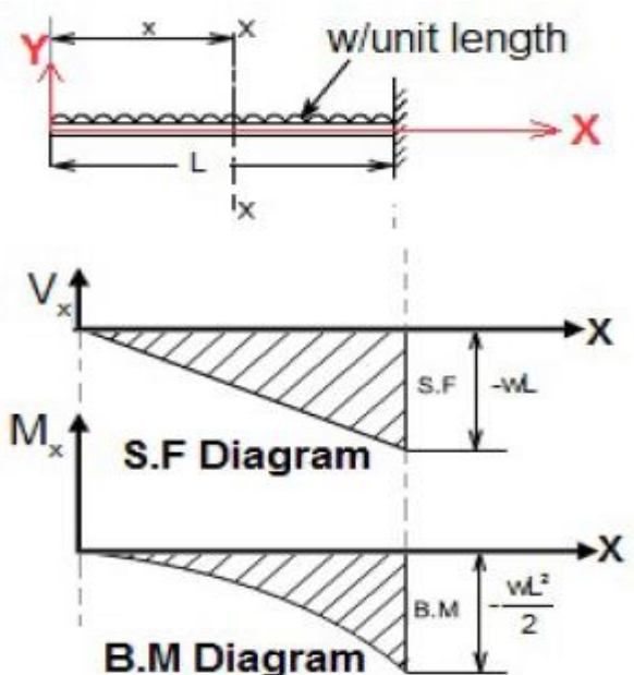
S.F and B.M diagram
